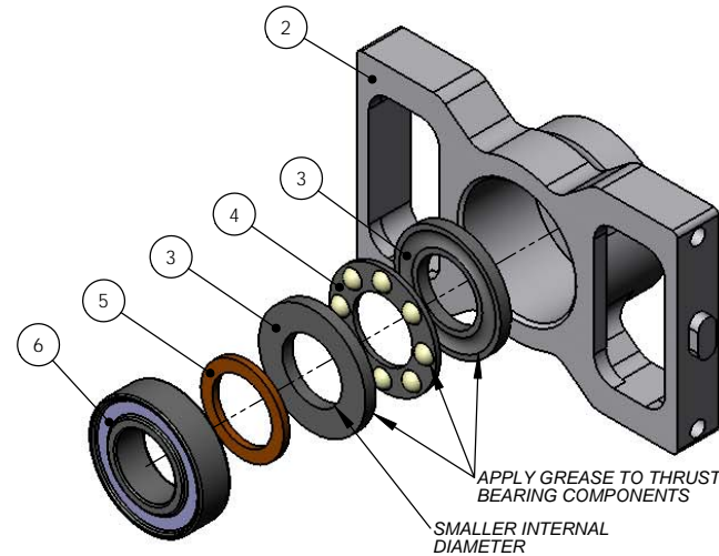
LOWER METAL BEARING BLOCK
